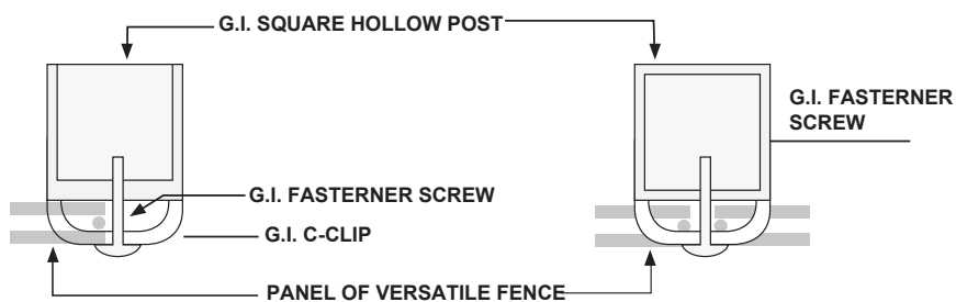
END POST
