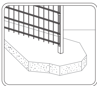
EMBEDDED POST
