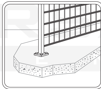
PLATED POST
