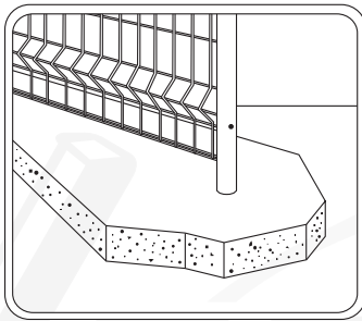
EMBEDDED POST
